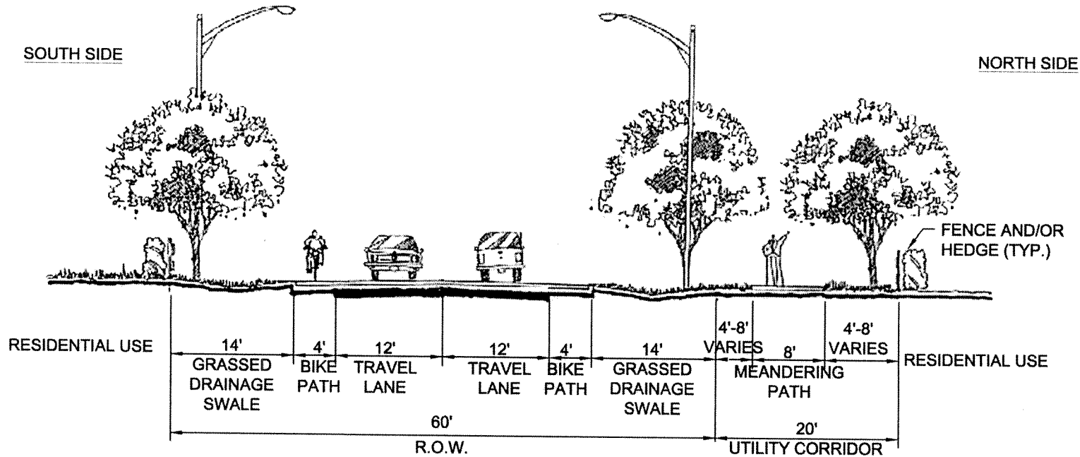
COUNTY STANDARD FOR COLLECTOR ROAD (*URBAN)
