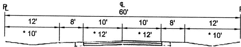
COUNTY STANDARD FOR COLLECTOR ROAD (*URBAN)
